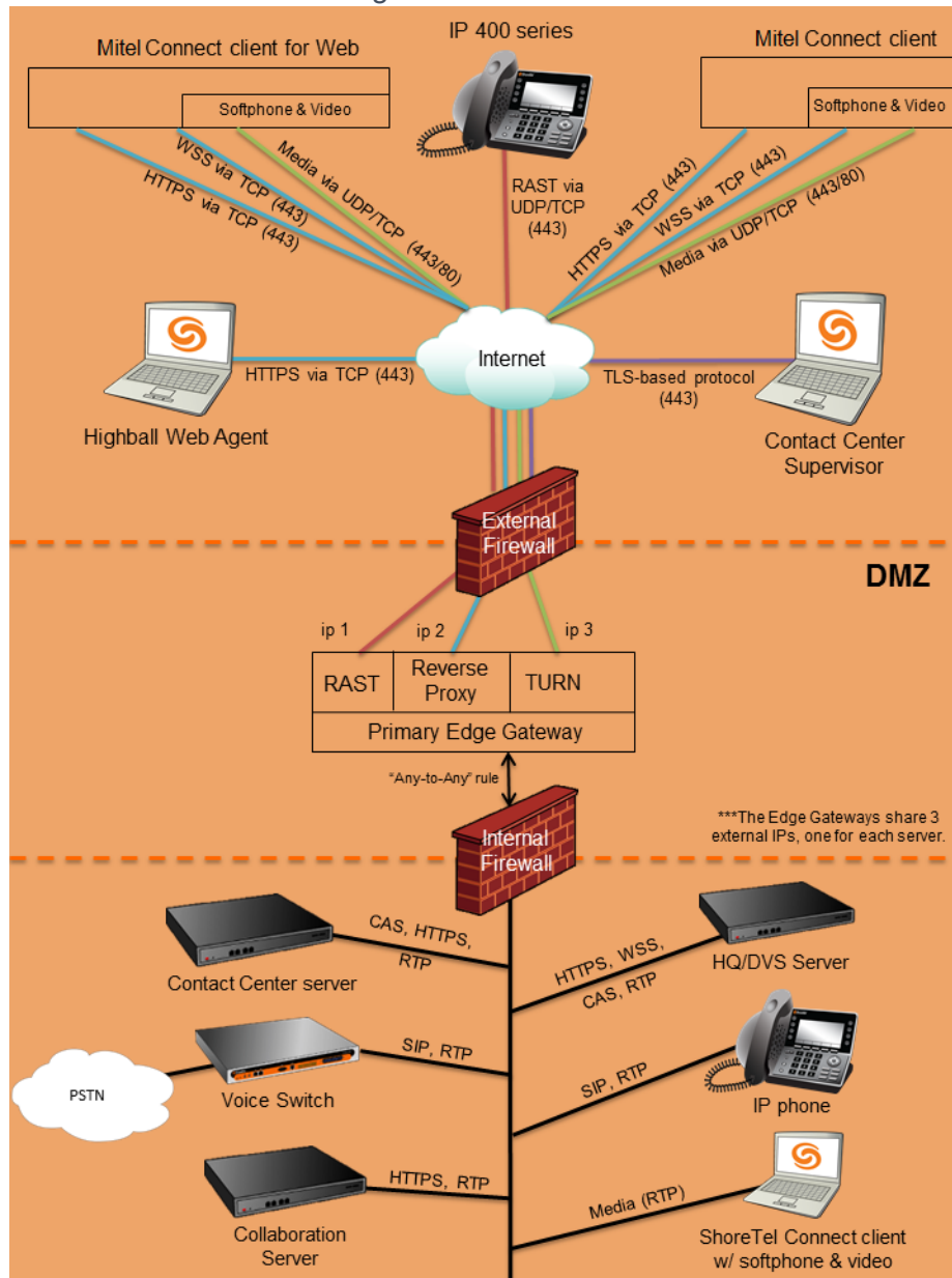
Figure 3.2: Network Architecture
